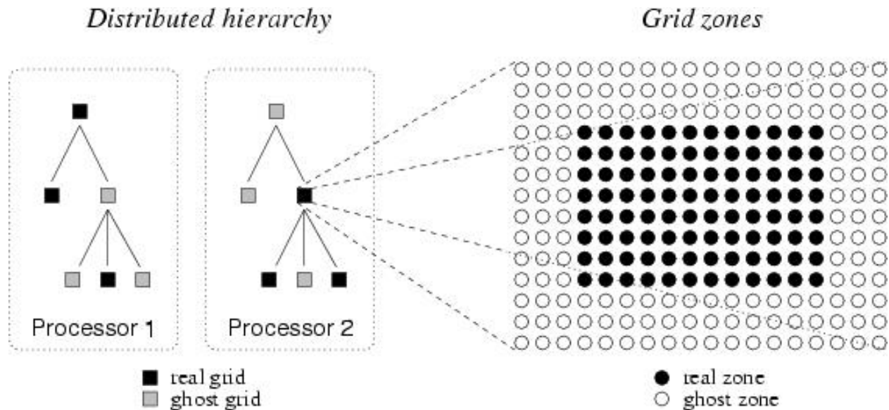
Fig. 7.1: Figure 1. Real and ghost grids in a hierarchy; real and ghost zones in a grid.
