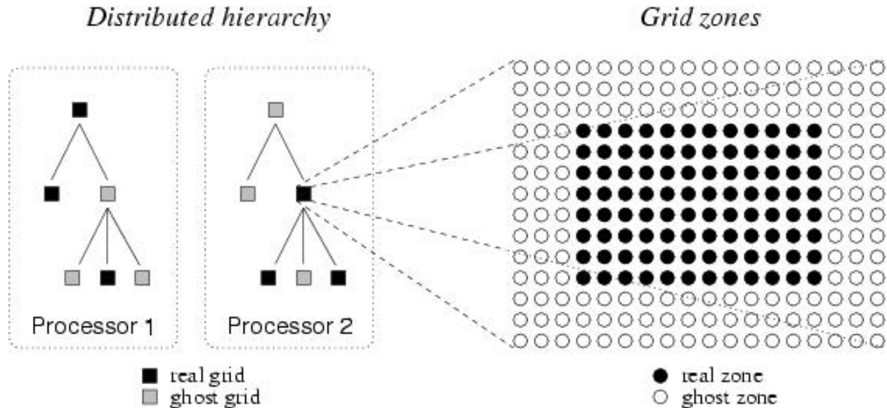
Fig. 1: Figure 1. Real and ghost grids in a hierarchy; real and ghost zones in a grid.
